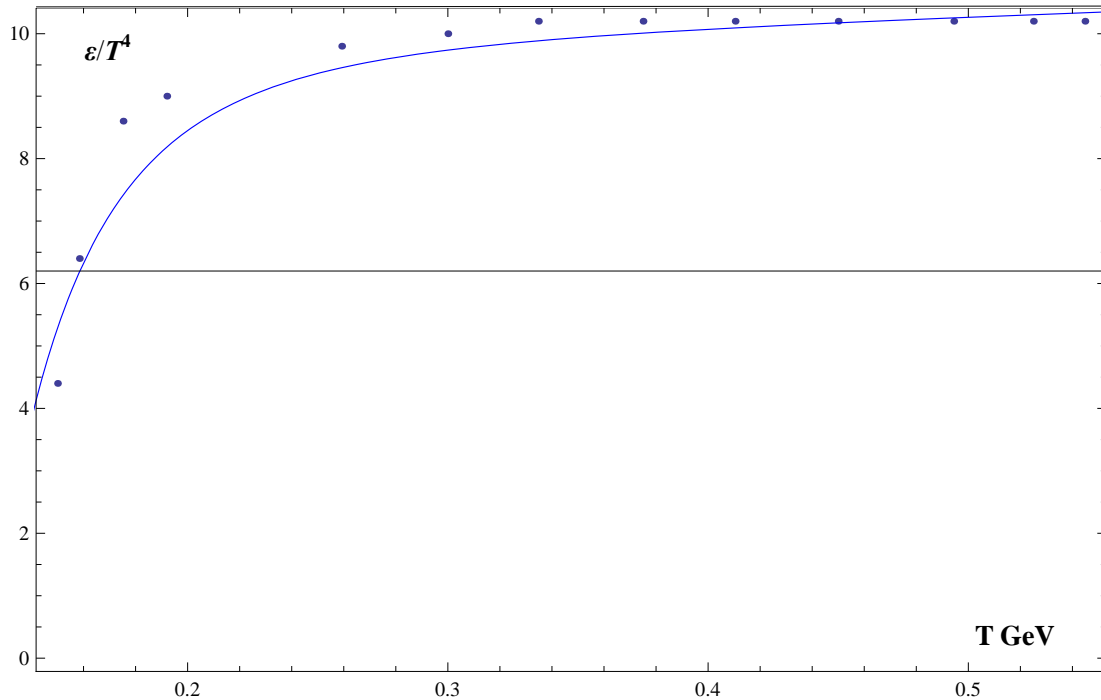
Figure 1. The solid curve gives the fitting of energy density normalized to T^4 from lattice QCD results for two flavors n_f = 2 .
