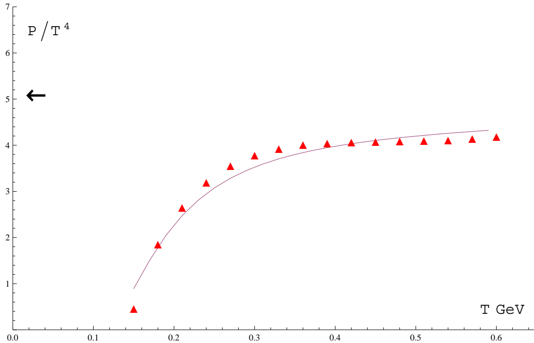
Figure 4. The solid curve gives the pressure normalized to T^4 comparing with lattice QCD results for two flavors n_f = 3 .
