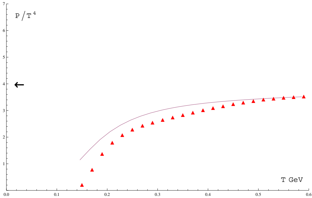
Figure 2. The solid curve gives the pressure normalized to T^4 comparing with lattice QCD results for two flavors n_f = 2 .
