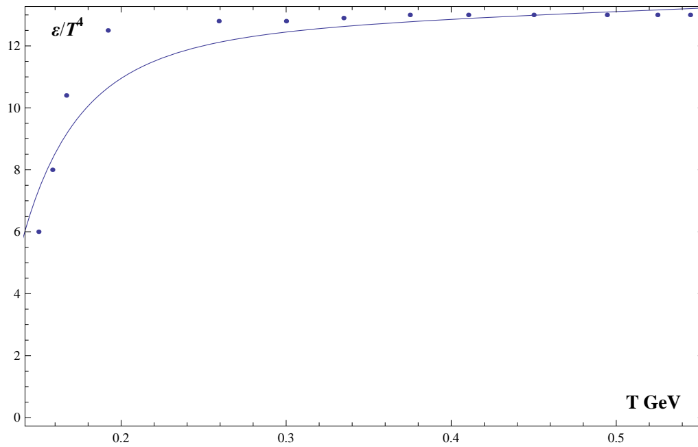
Figure 3. The solid curve gives the fitting of energy density normalized to T^4 from lattice QCD results for three flavors n_f = 3 .
